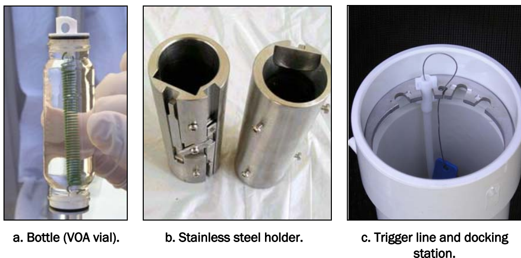
Figure 1. Snap Sampler.
